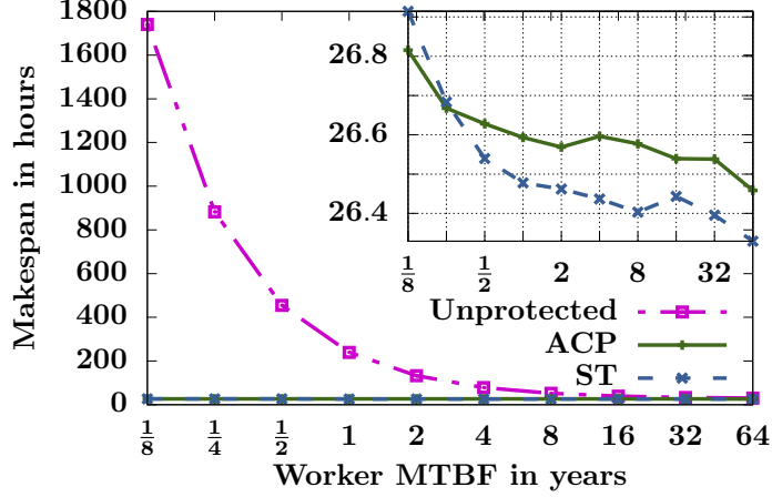
Figure 8: Mira simulation
